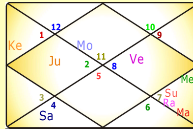
Moon Chart
