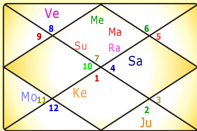
Lagna Chart
