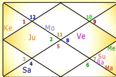
Moon Chart
